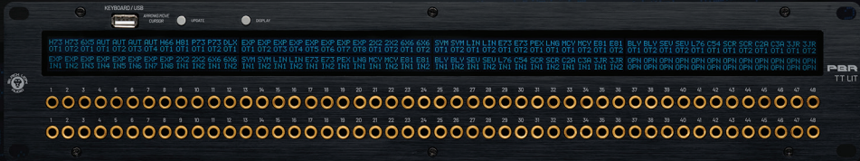
PBR TT LIT: 96-point TT/DB25 patchbay with LED display system, audiophile-grade jacks, and 3 normalization modes.
